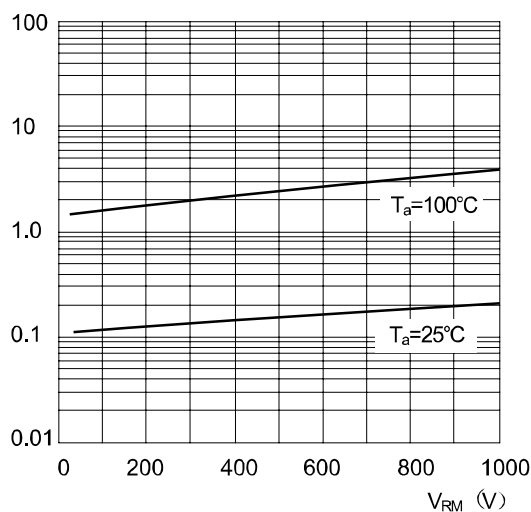
Reverse Characteristics
